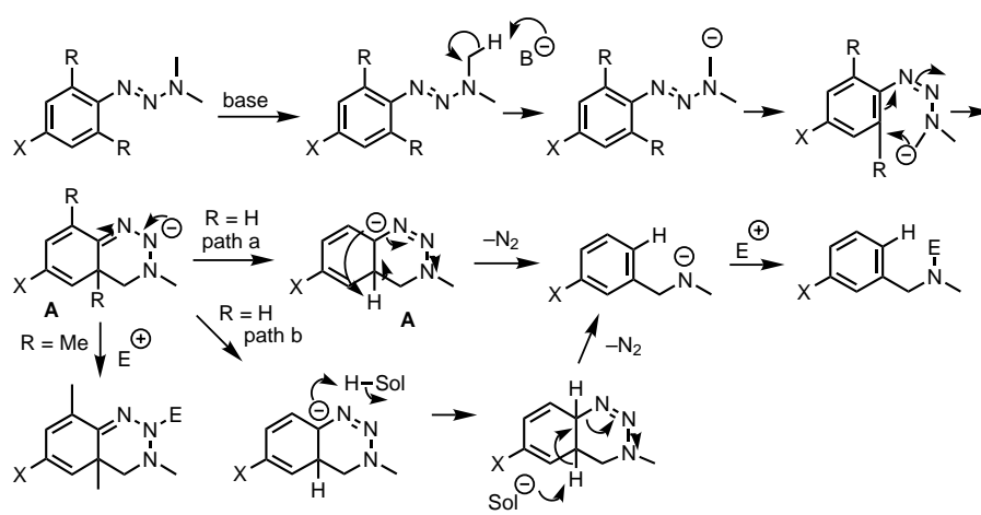
Scheme 2. Proposed mechanism.
